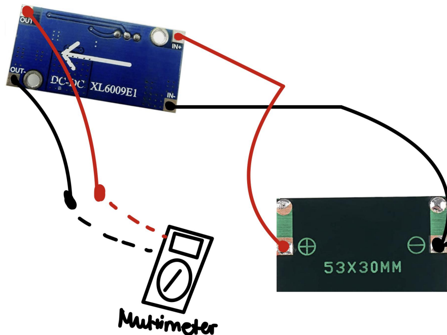
Figure 44: DC to DC Testing
