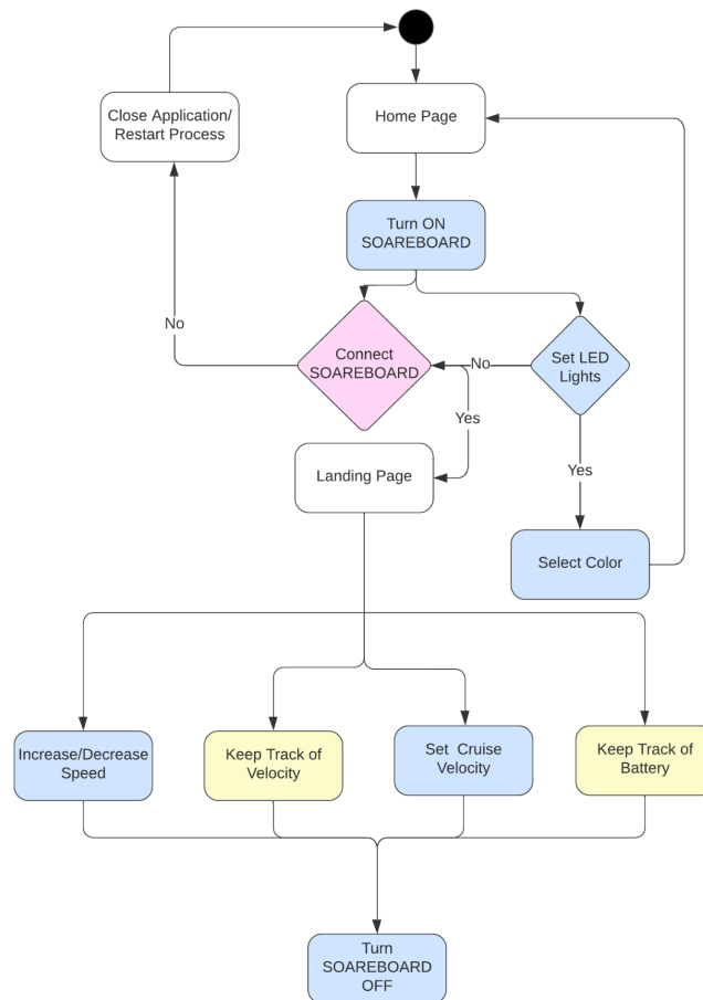
Figure 43: App and MCU Interaction Activity Diagram
