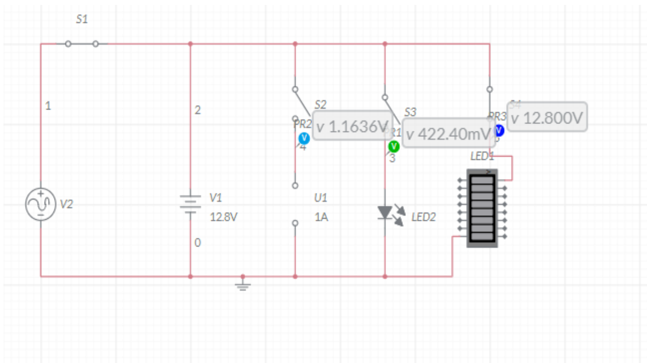
Figure 28: Schematic Simulation
