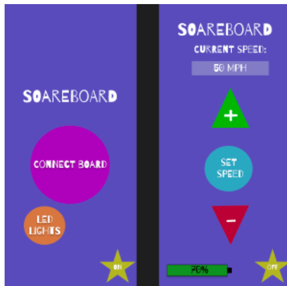
Figure 39: App Design
