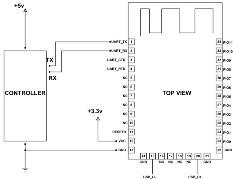
Figure 11: Schematic of HM-10 BLE Connection to Microcontroller
