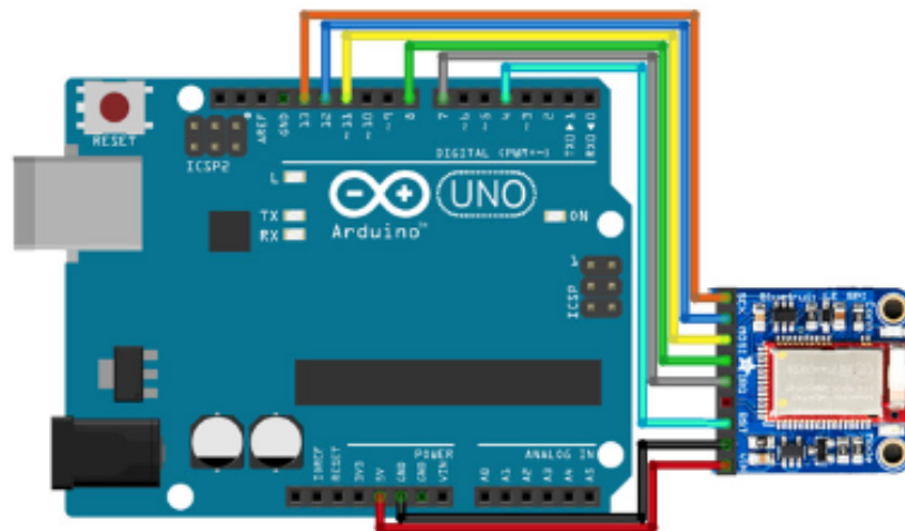
Figure 12: Bluefruit LE SPI Friend Module Connection with Arduino UNO
