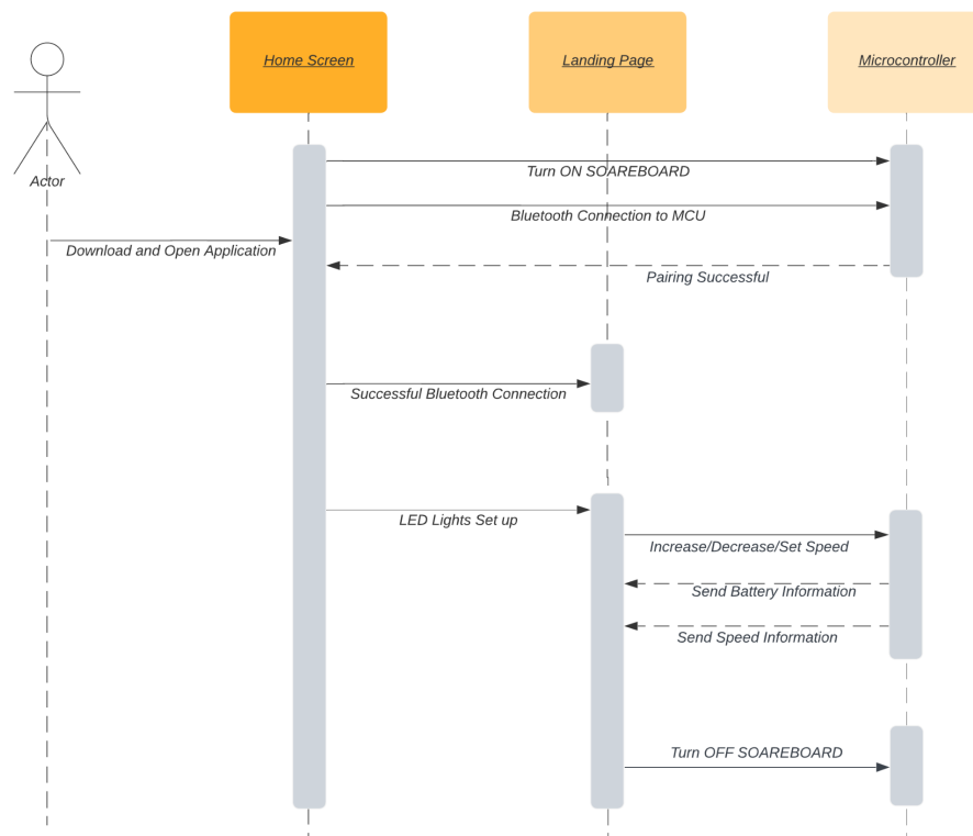
Figure 41: Sequence Diagram
