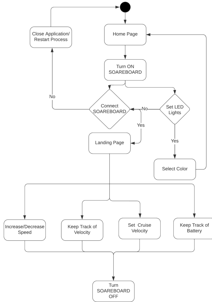
Figure 38: Activity Diagram
