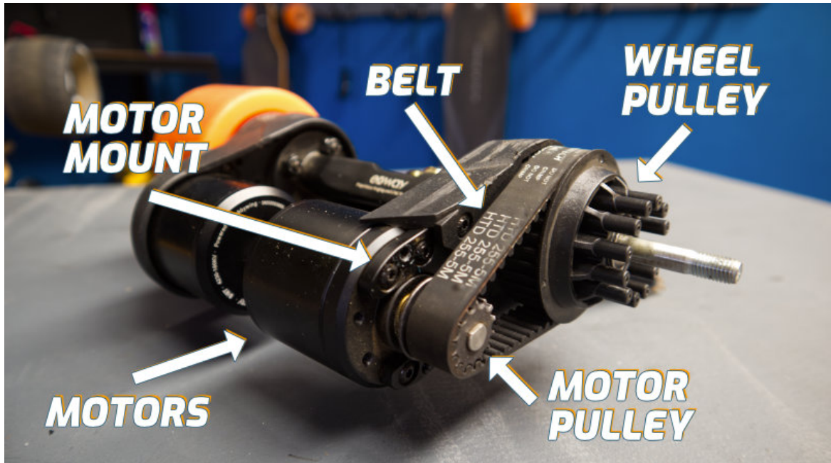
Figure 16: Driving System Component Breakdown
