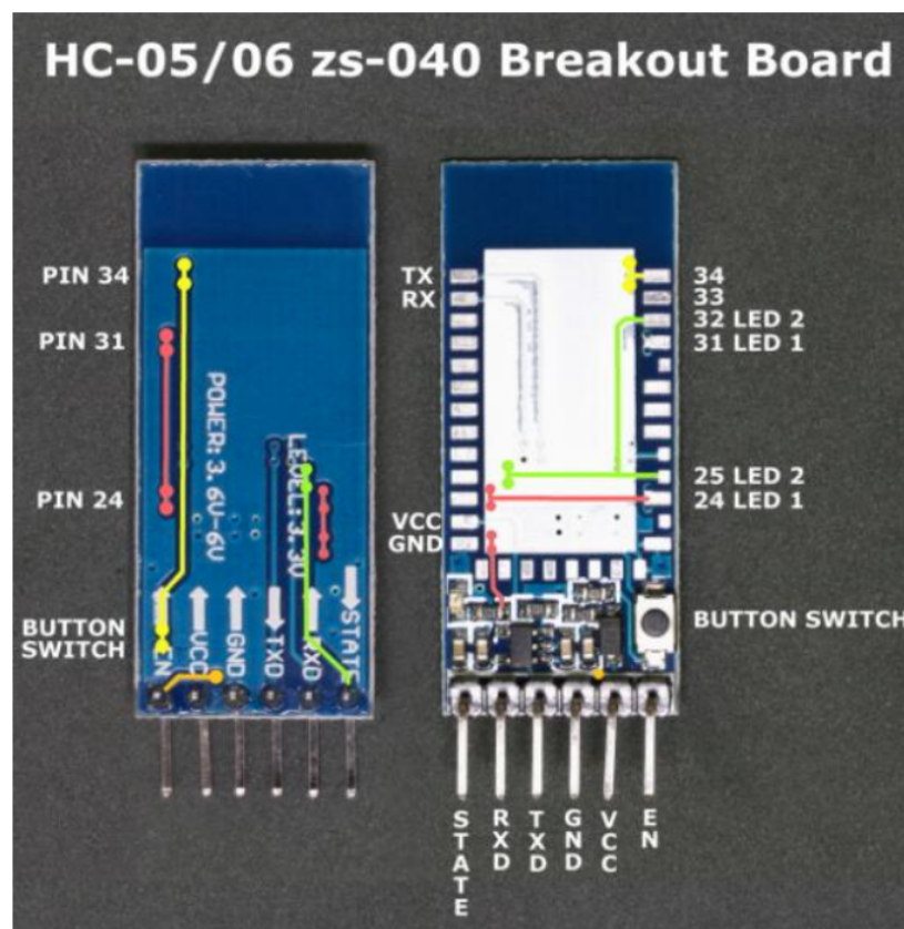
Figure 10: Pinout of HC-05/HC-06 Bluetooth Modules
